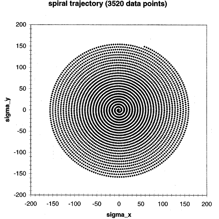
Fig. 2. Trajectory in k -space in the case of one-interleave spiral imaging with 3520 data points.
