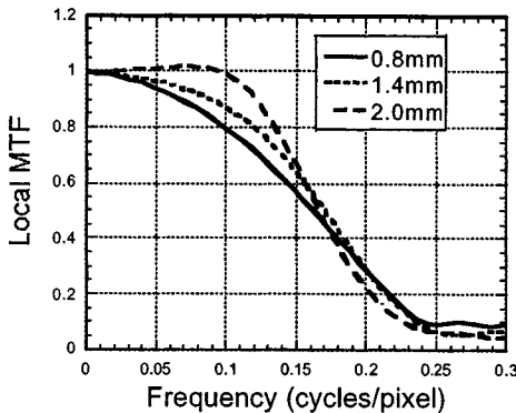
Fig. 10. Radially averaged profiles through the MTF_r for compensations at 0.8, 1.4, and 2.0 mm after 200 Landweber iterations.
