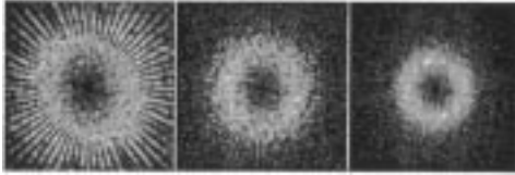
Fig. 8. W_r for (from left to right) 0.8-, 1.4-, and 2.0-mm assumed bore diameters after 200 iterations for ML-EM reconstruction of a uniform disk.
